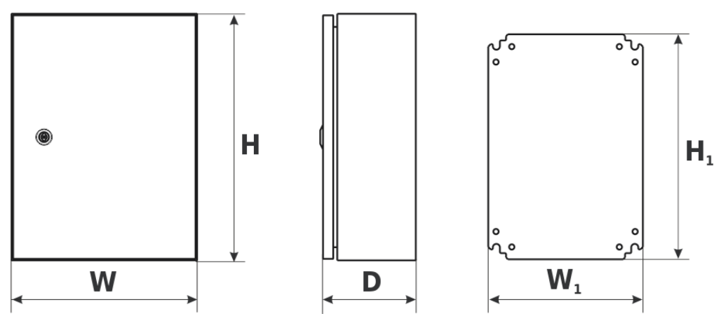
Fig. 2. Dimensions.
